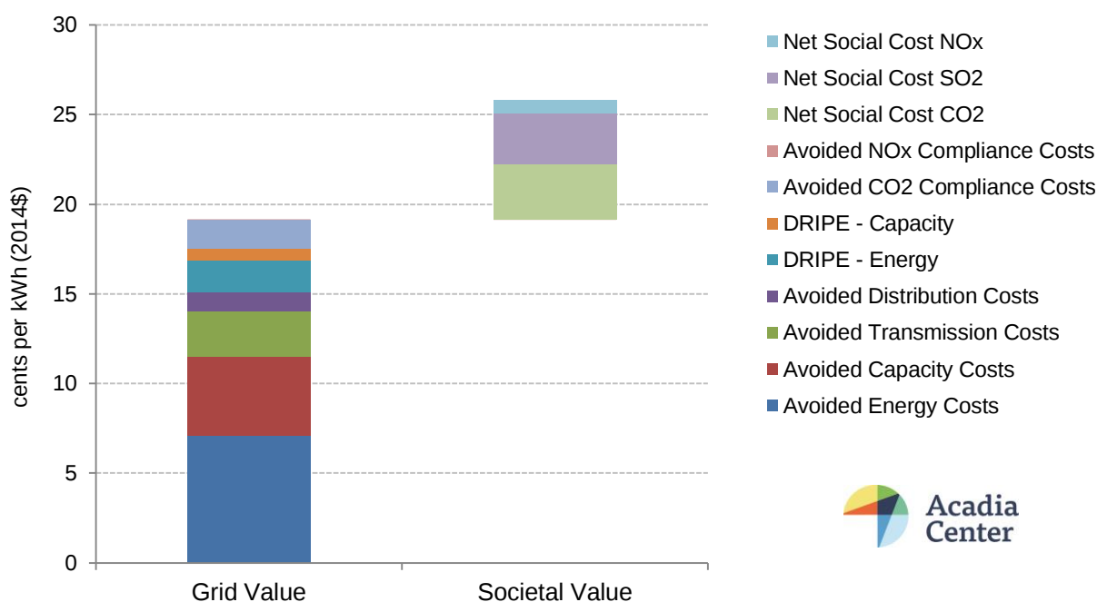
Figure 1: Grid and Societal Value of Solar PV in New Hampshire – 25-year Levelized Cost (2014$)
